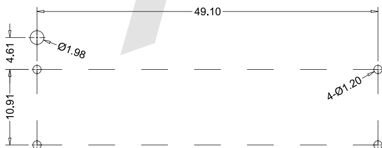
MOUNTING PAD LAYOUT
